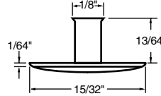
106-W05-1K EYELET
