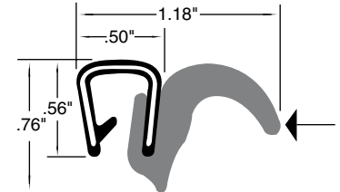
825-301 Lip Seal
