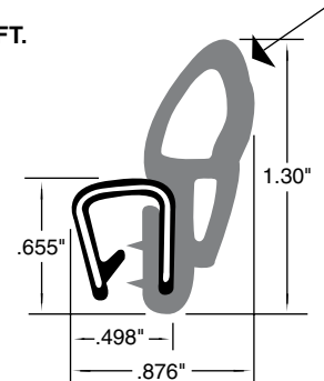
825-303 Vertical Wedge
