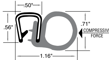
825-B18-1K Bulb Seal
