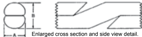
Enlarged cross section and side view detail.
