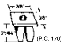
B-1576 Screw Size #8 or 10 Panel Hole .275-.280" sq. Panel Range .040-.045"
