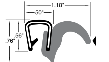
825-301 Lip Seal
