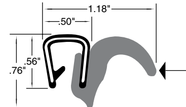
825-301 Lip Seal
