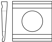
DIN 434 Square Beveled Washers – 8% Slope for “U” Beams Plaquettes obliques carreau pg. D76
