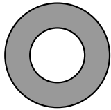
DIN 433 Flat Washers with reduced O.D. Rondelles en acier pg. D17 ~ISO 7092
